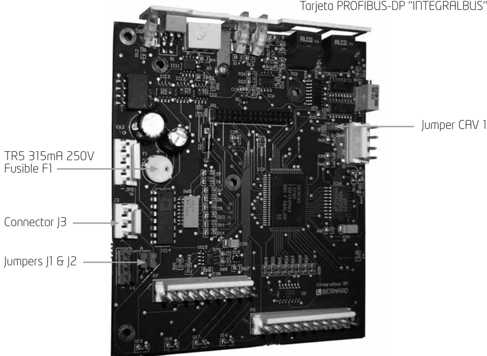
Tarjeta PROFIBUS-DP "INTEGRALBUS"
