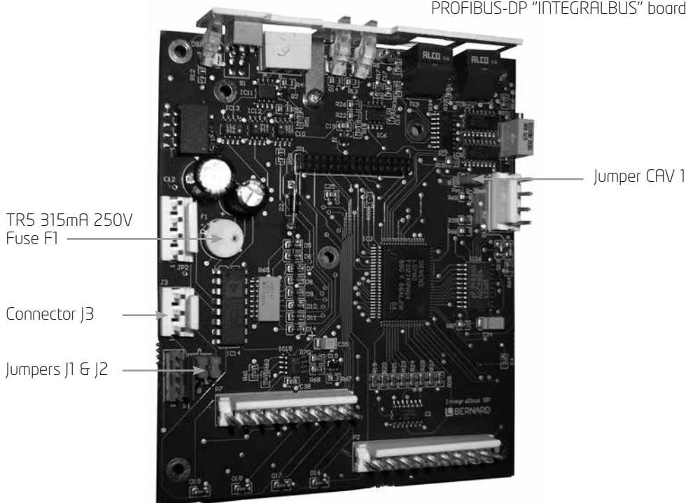
PROFIBUS-DP "INTEGRALBUS" board
